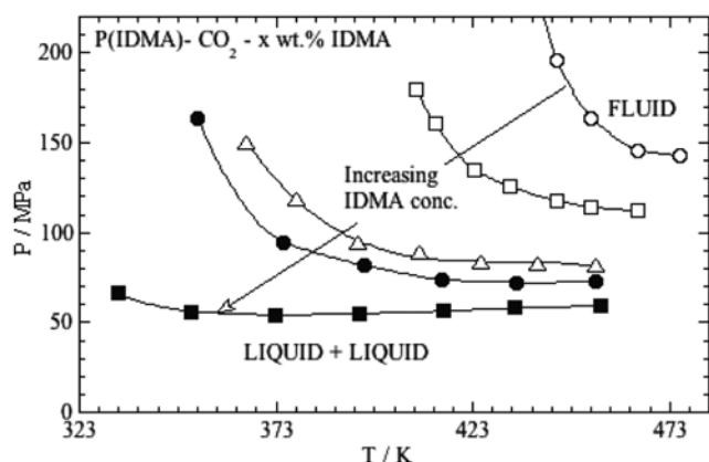
Fig. 1. Experimental cloud-point curves for the poly(isodecyl methacrylate) [P(IDMA)]+CO 2 +isodecyl methacrylate (IDMA) system with different IDMA concentrations. The polymer concentration is ca. 5 wt% for each solution. ○, 0.0 wt%; □, 6.0 wt%; △, 16.3 wt%; ●, 28.0 wt%; ■, 45.5 wt%.
